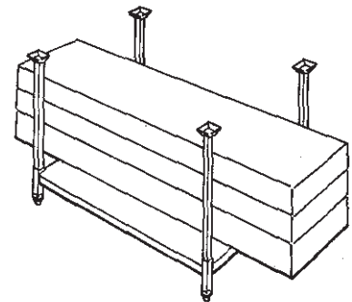
Long, evenly distributed load with overhanging ends. "OK"
