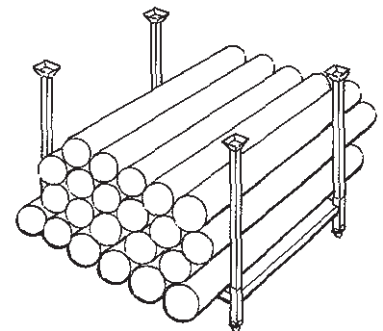
Loose load is not self contained, and applies considerable pres- sure to corner columns. "May Require Special Design"
