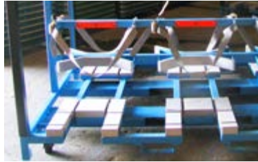
Fuel tank rack
