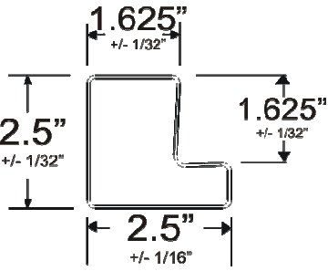
2.5" Step Beam
